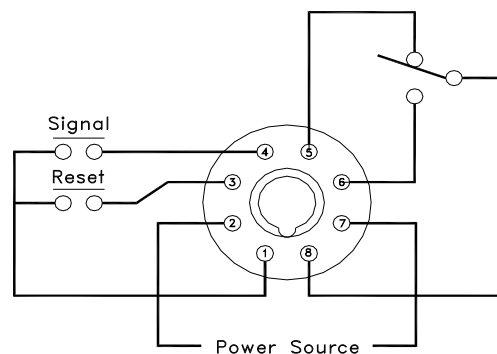
DET1 Back Panel Controls and Wiring Diagram
